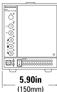
Front Panel
